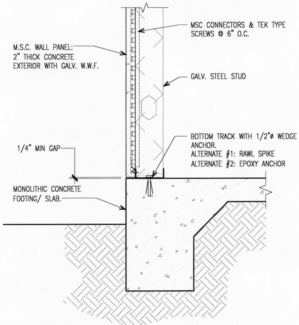
TYPICAL M.S.C. WALL TO FOUNDATION SLAB
