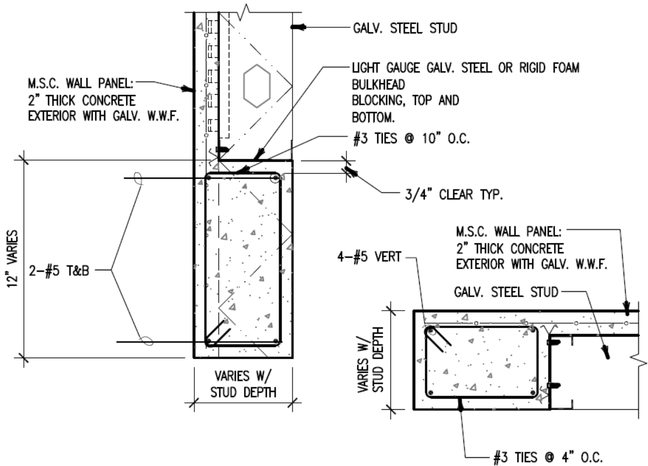
HEADER SECTION
