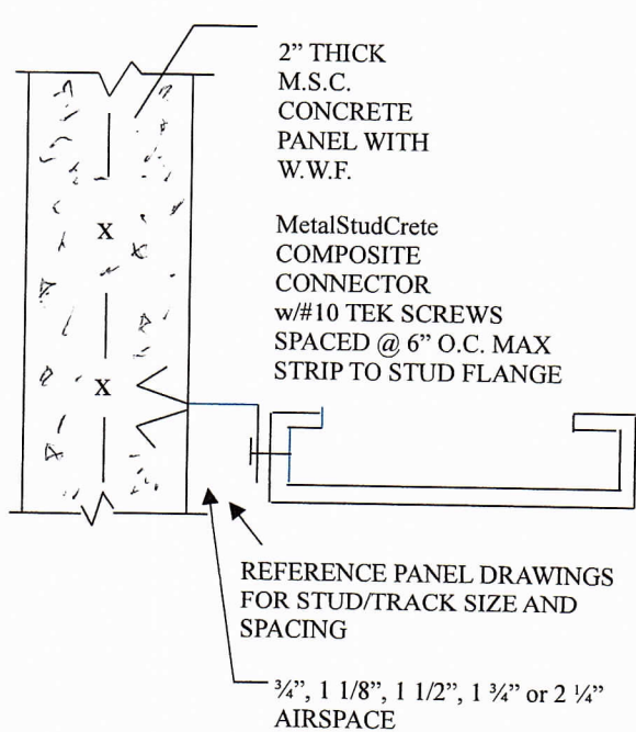
5 MC10 M.S.C. TRANSFER STRIP @ STUD/TRACK FLANGE
